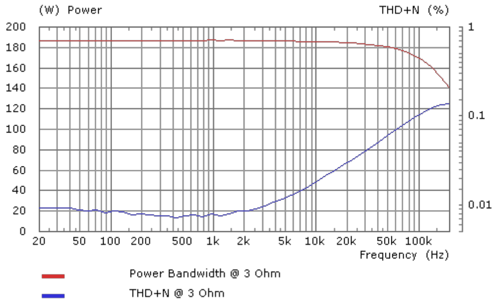
Power bandwidth at 3 Ohm load (Input level normalized to max. output level at 200 kHz; THD+N < 1%)
