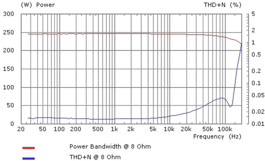
Power bandwidth at 8 Ohm load (Input level normalized to max. output level at 200 kHz; THD+N < 1%)
